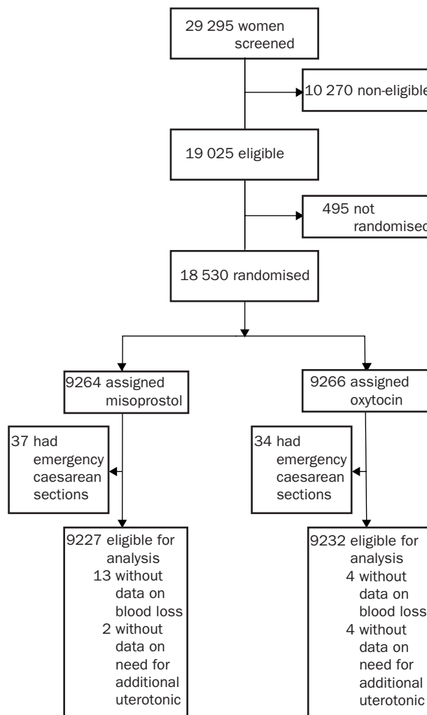
Figure 1: Trial profile
